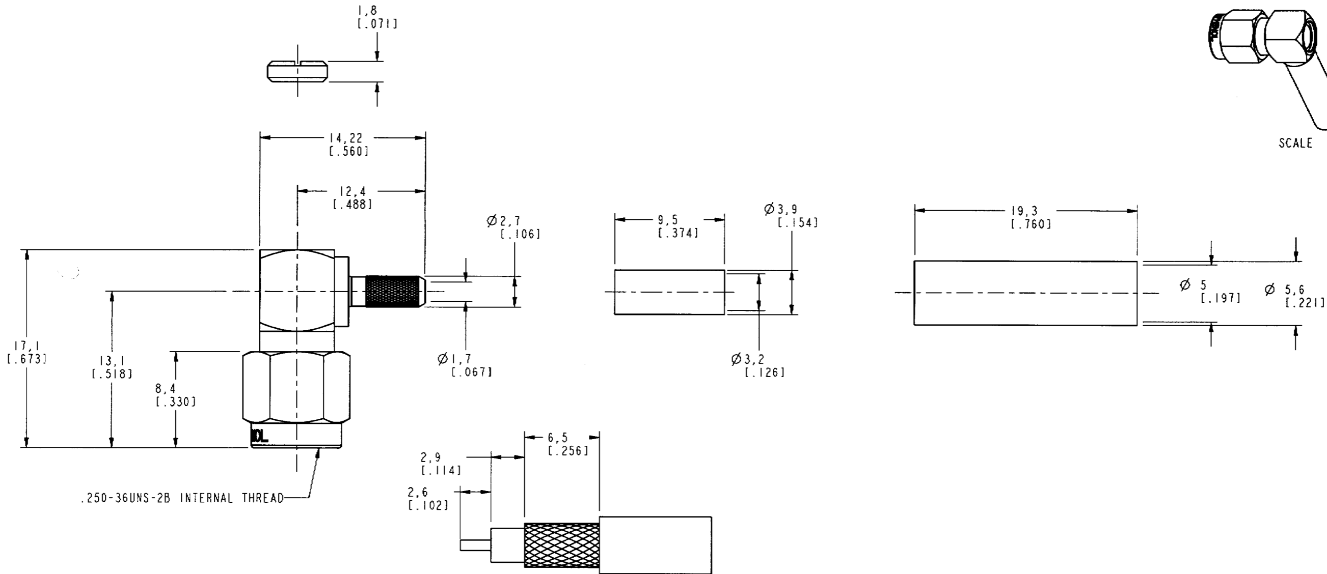
RECOMMENDED CABLE STRIPPING DIMENSIONS SCALE 3.000
