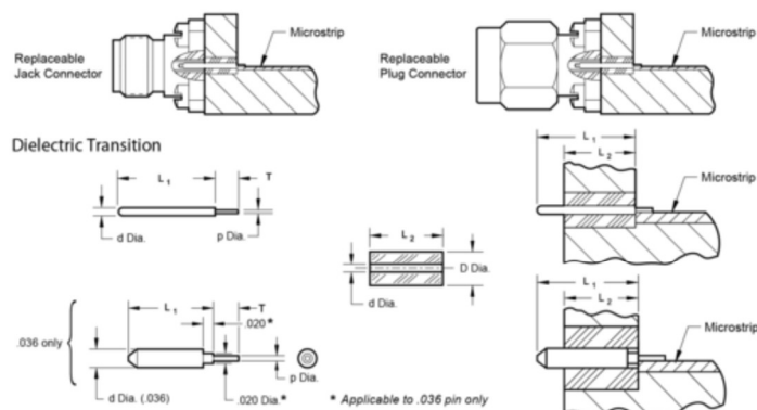
Launch Pin and Dielectric Transition to Microstrip
