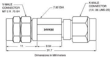
34VK50 outline
