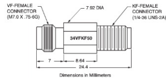
34VKF50 outline
