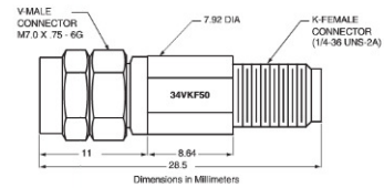
34VKF50 outline
