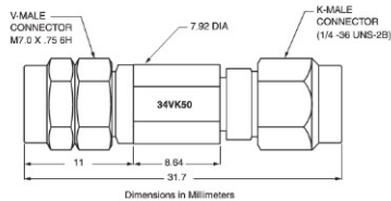
34VK50 outline
