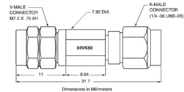
34VK50 outline
