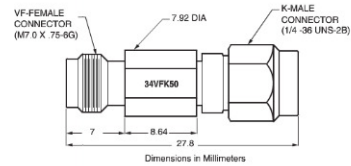
34VK50 outline
