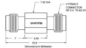
34VVF50 outline
