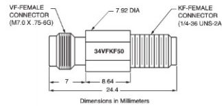
34VKF50 outline
