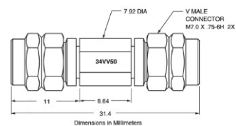
34VV50 outline
