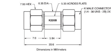
K220B outline
