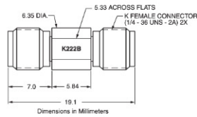
K222B outline
