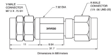
34VK50 outline
