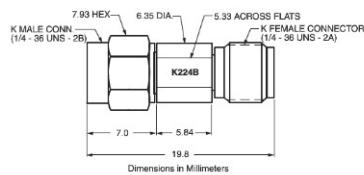
K224B outline
