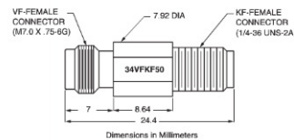
34VFKF50 outline
