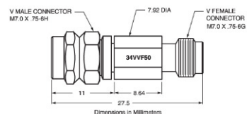
34VVF50 outline
