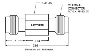
34VVF50 outline
