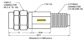
34VKF50 outline
