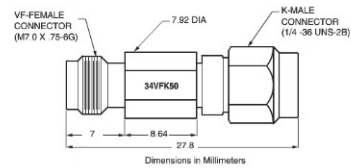
34VFK50 outline
