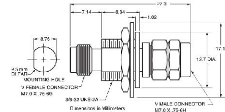
V234 outline
