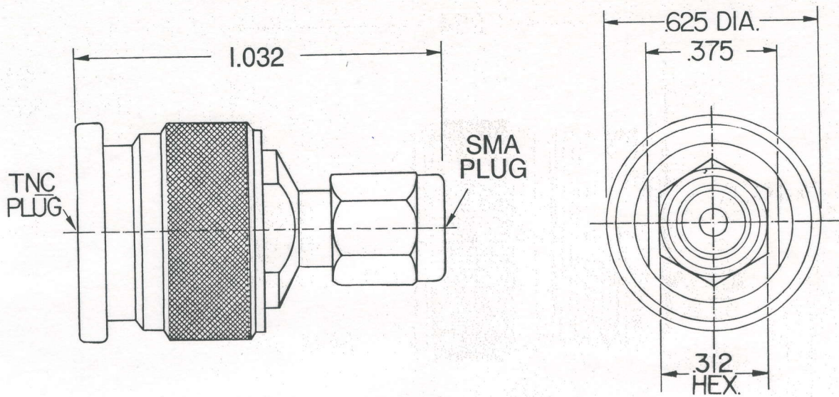
7006 TNC PLUG TO SMA PLUG
