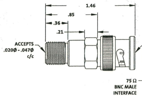
BNC Male - F Female Adapter
