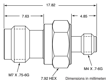
34WV50 outline
