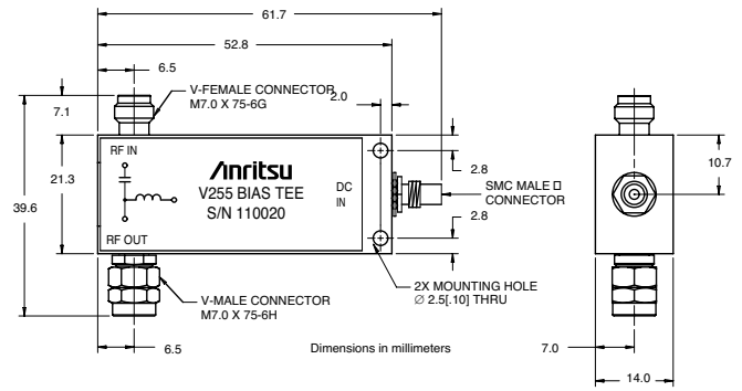
V255 outline
