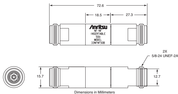
33NKF50B outline
