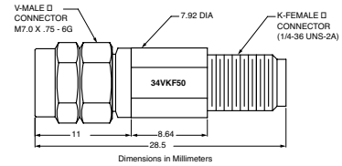
34VKF50 outline
