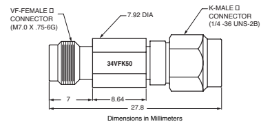
34VFK50 outline
