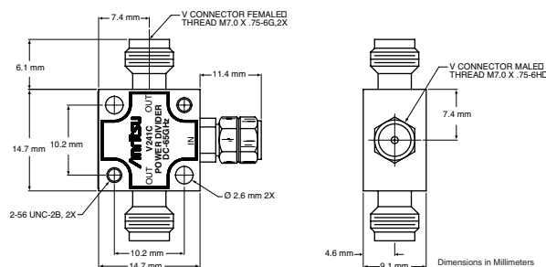
V241C outline
