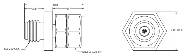
W1 Female to 0.8 mm Male Adapter (33WF.850)
