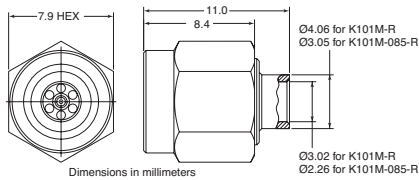
K101M-R ④⑥ K Male In-Line Cable Connector, DC-40 GHz for 2.95 mm cable K101M-085-R ④ for 2.18 mm cable
