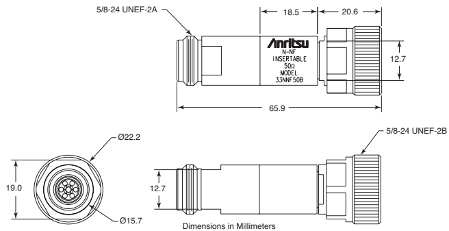
33NNF50B outline
