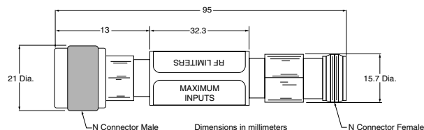
IN50C and IN75C Limiters outline
