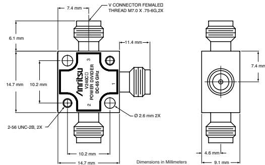
V240C outline
