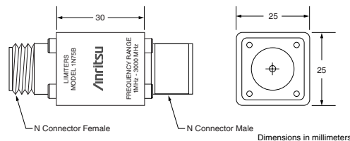
IN50B and IN75B Limiters outline
