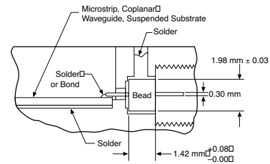
Transition from Microcircuit to External Transmission Line
