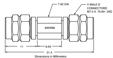
34VV50 outline
