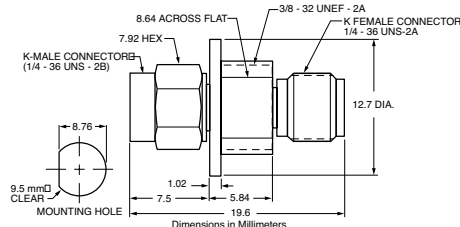
K234B outline
