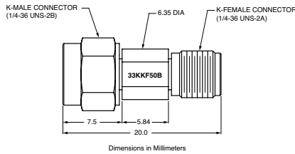
33KKF50B outline
