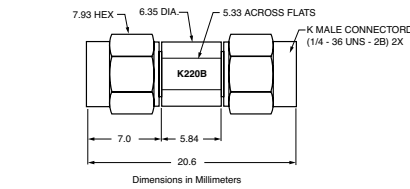
K220B outline
