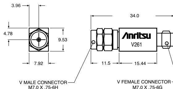
V261 outline
