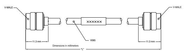
V120MM outline
