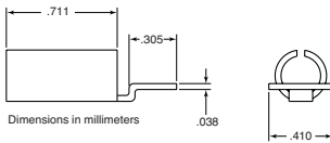
K110-2-R ® Stripline
