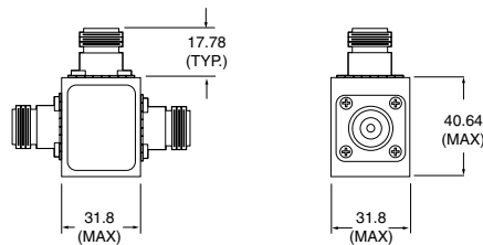
N241A50 outline
