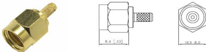
Straight Cable Plug
