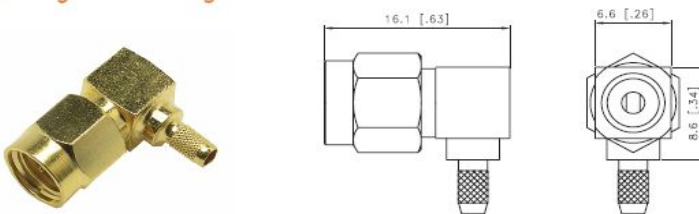
Right Angle Cable Plug
