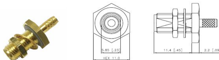
Bulkhead Cable Jack
