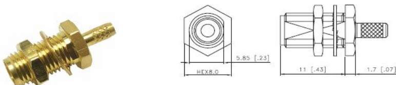
Bulkhead Cable Jack
