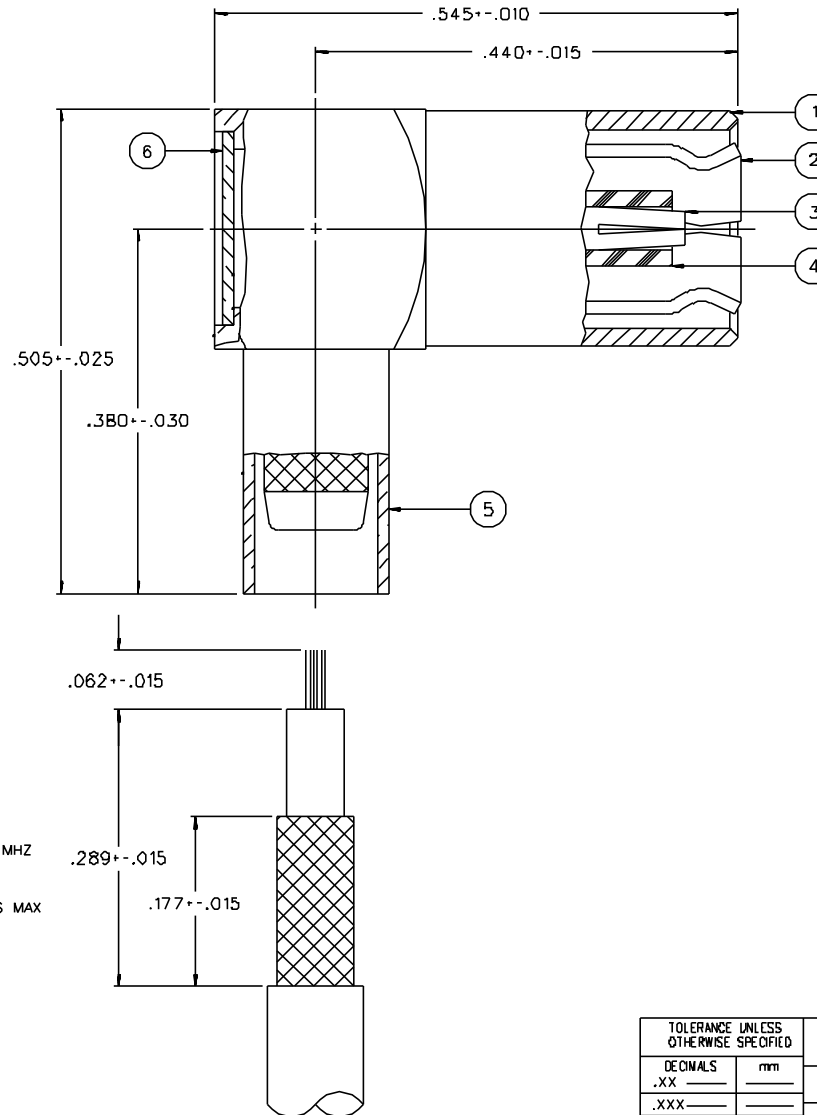
CABLE STRIP DIMENSIONS
