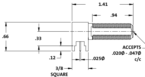
Standard Right Angle PCB Mount
