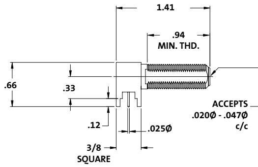
Long Right Angle PCB Mount
