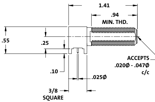
Low Profile Right Angle PCB Mount
