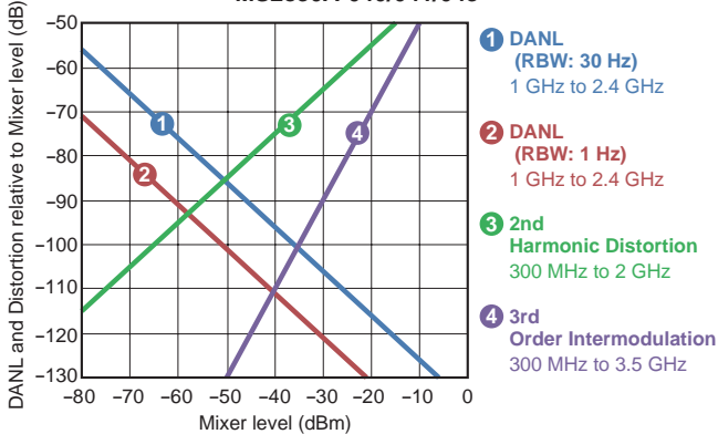
Distortion Characteristics (Spectrum Analyzer) MS2830A-040/041/043
